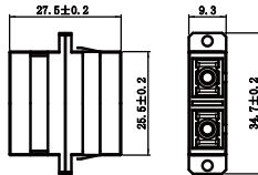
SC DX Welding Adaptor With Flange
