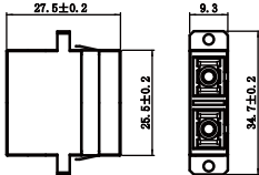
SC DX One-piece Adaptor With Flange
