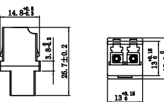
LC DX High-Low Adapter
