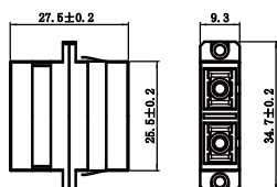
SC DX Metal Adaptor
