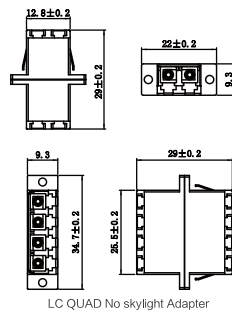
LC QUAD No skylight Adapter
