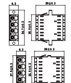
LC QUAD One-piece Adapter Without Flange
