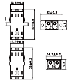
LC DX One-piece Adapter Without Flange
