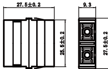
SC DX Welding Adaptor Without Flange
