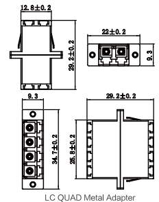
LC QUAD Metal Adapter
