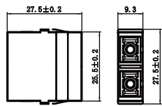
SC DX One-piece Adaptor Without Flange
